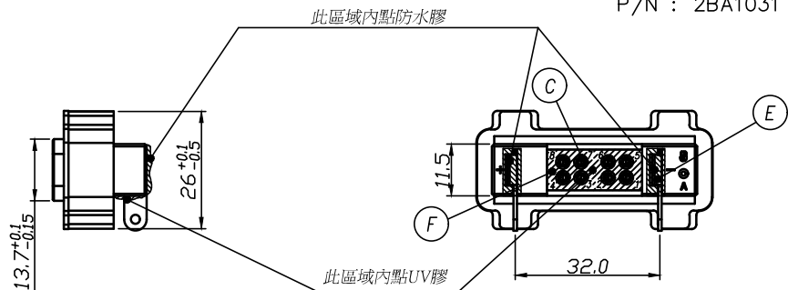
MATING PART P/N : 2BA1031 SERIES
