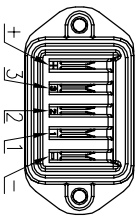
Pin Assignments Front View
