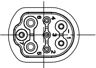
PIN ASSIGNMENTS FRONT VIEW
