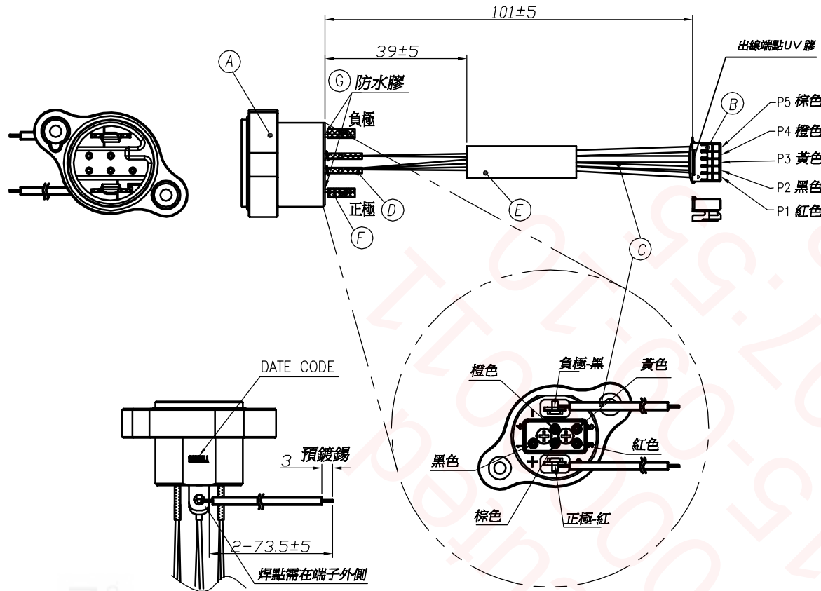
BATTERY CONNECTOR WIRE DIAGRAM CONNECTOR(A)
