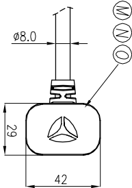
CONN2&3 BACK VIEW
