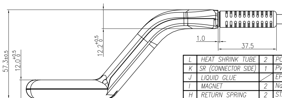
POWER CONNECTOR
