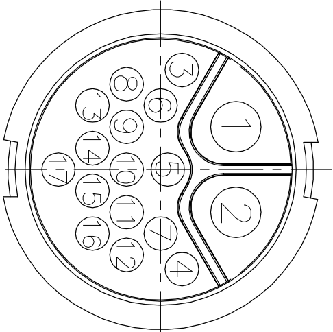
Pin Assignments Front View 前視圖
