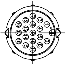
Pin Assignments Front View 前视图
