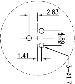
3 PIN MALE CONNECTOR MALE PIN PCB LAYOUT
