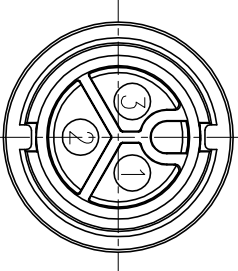
Pin Assignments
