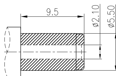
PLUG DIAGRAM (TOL: ±0.05[±0.002] )
