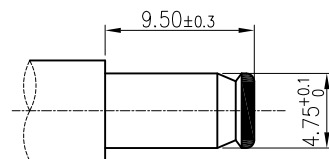
MATE PLUG
