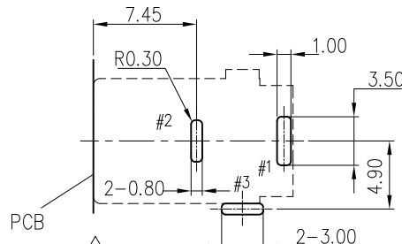
RECOMMENDED PCB LAYOUT (TOP VIEW)(TOL.:±0.05)
