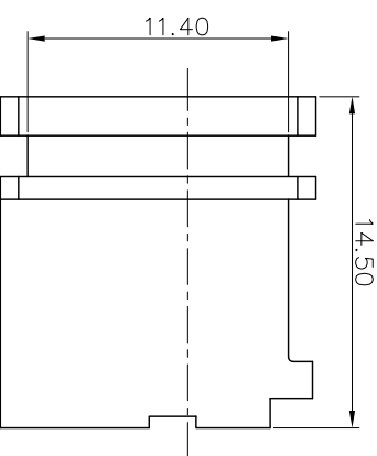
MATING PLUG ø5.50
