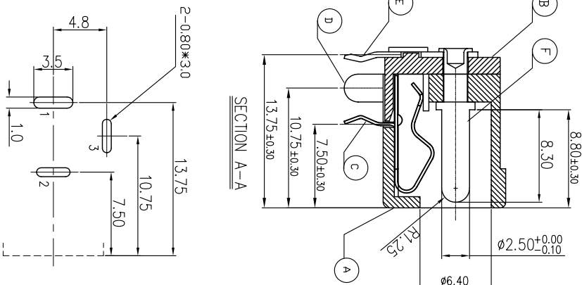
RECOMMENDED P.C. BOARD LAYOUT (TOP VIEW)(TOL. ±0.05)
