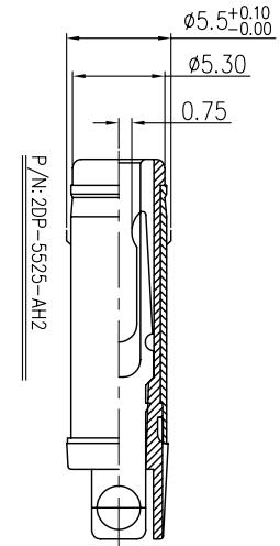
MATING PLUG(REF ONLY)
