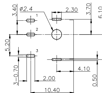
RECOMMENDED P.C.B LAYOUT TOP VIEW (TOLERANCE: ±0.05)
