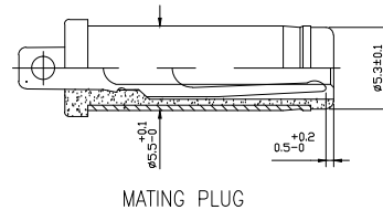
MATING PLUG
