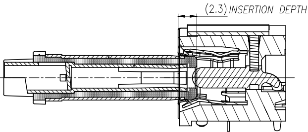
1. GROUNDING CONTACT FIRST
