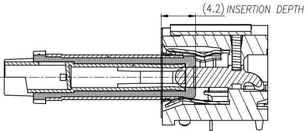
3. POSITIVE CONTACT
