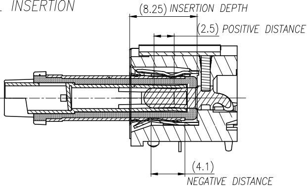
5. FULL INSERTION
