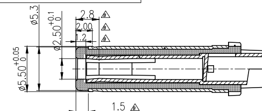
MATING PLUG (TOLERANCES: ±0.10)
