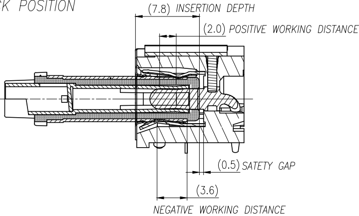
4. LOCK POSITION
