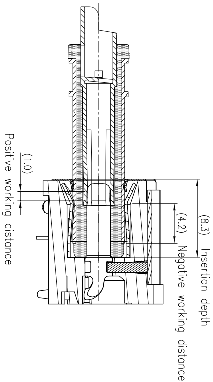
4. FULL INSERTION
