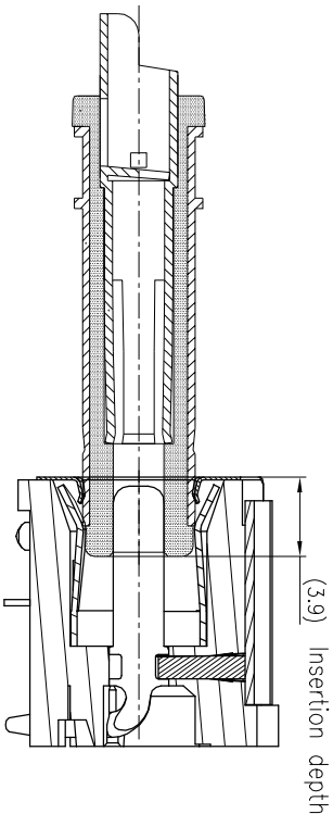
2. SPRING- CONTACT
