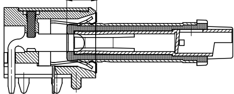
3.PIN(+) CONTACT
