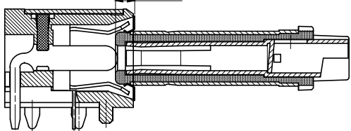
1.GROUND CONTACT
