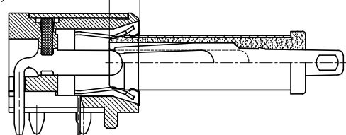
2.PIN(+) CONTACT
