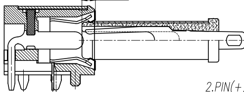
2.PIN(+) CONTACT
