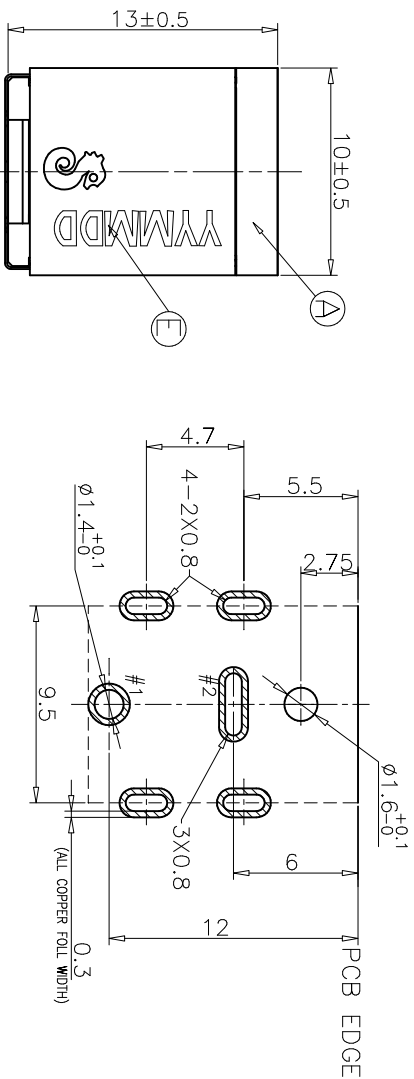
RECOMMEND P.C.B LAYOUT TOP VIEW(TOLERANCE ±0.05)
