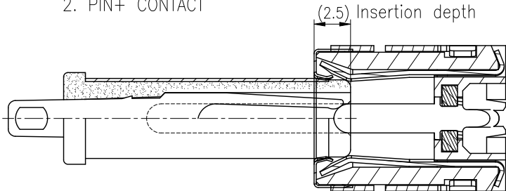
2. PIN+ CONTACT
