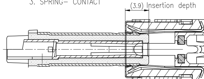
3. SPRING- CONTACT
