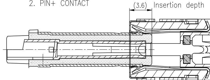
2. PIN+ CONTACT
