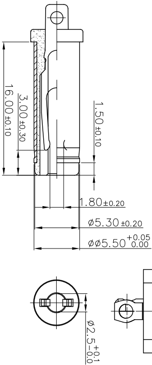
MATING PLUG Ø5.50
