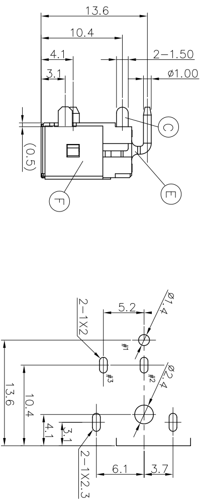
RECOMMEND P.C.B LAYOUT TOP VIEW (TOLERANCES:±0.05)
