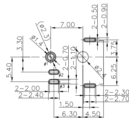
RECOMMENDED P.C.B LAYOUT TOP VIEW (TOLERANCES:±0.05)
