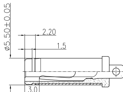
MATING PLUG \phi 5.50
