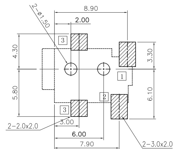
Recommend of PC Board Holes
