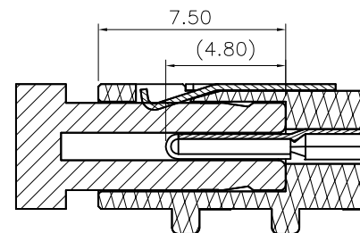
Plug Matching Diagram
