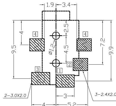
T:1.6 Dimensions of PC board holes
