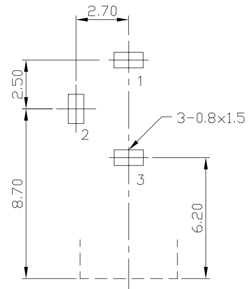
P.C.B LAYOUT( \pm 0.1 ) (BOTTOM VIEW)
