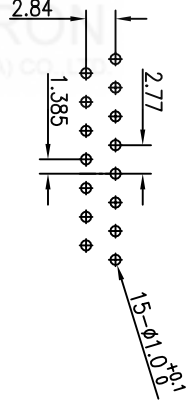
15 PIN FEMALE CONNECTOR PCB PIN LAYOUT
