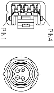
Pin Assignments Front View
