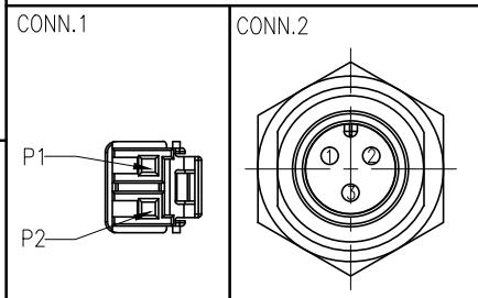
Pin Assignments Front View
