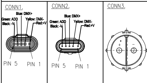
Pin Assignments Front View
