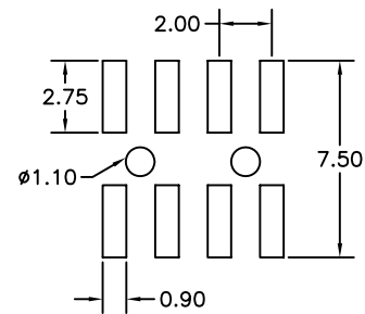
Recommended P.C.Board SMD Layout
