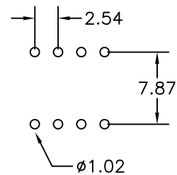
Recommended P.C.Board Hole Layout
