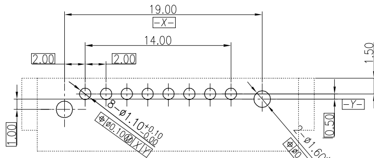
RECOMMENDED P.C.B LAYOUT(TOP VIEW) TOLERANCE ±0.05mm(T=1.20mm)
