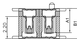
Mating Drawing (Ref)
