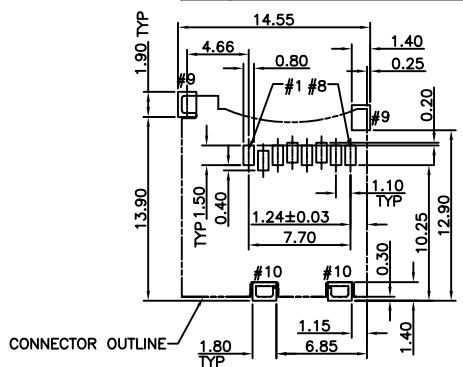
CONNECTOR OUTLINE RECOMMENDED PCB PATTERN LAYOUT TOLERANCE: ±0.05
