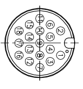
Pin Assignments Front View 前視圖
