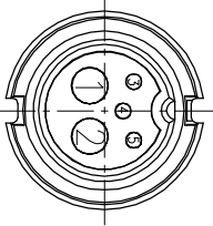
Front View Pin Assignments
