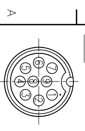
Pin Assignments Front View
