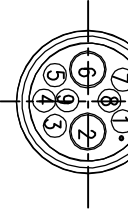
Pin Assignments Front View
