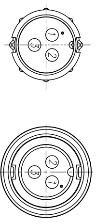
Pin Assignments Front View Pin Assignments Front View
