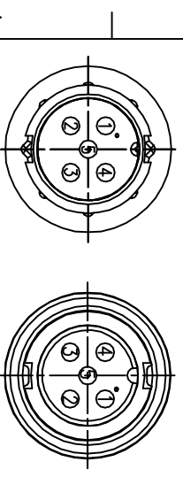
Pin Assignments Front View
