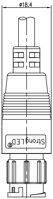
A VIEW
