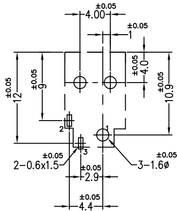
RECOMMENDED P.C.B LAYOUT SOLDER SIDE
