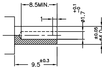
MATE PLUG
