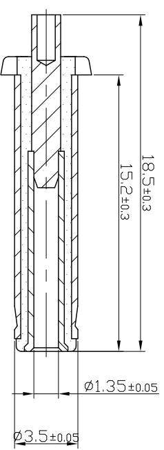
MATING PLUG: OD0.3.5 x ID0.1.3 PLUG
