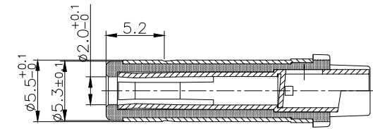
MATING PLUG (TOLERANCE: ±0.05)
