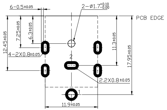
RECOMMENDED P.C.B LAYOUT SOLDERING SIDE
