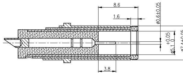
MATING PLUG TOLERANCE:±0.10
