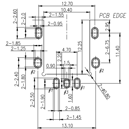
RECOMMEND PCB LAYOUT TOP VIEW(TOLERANCES:±0.05)
