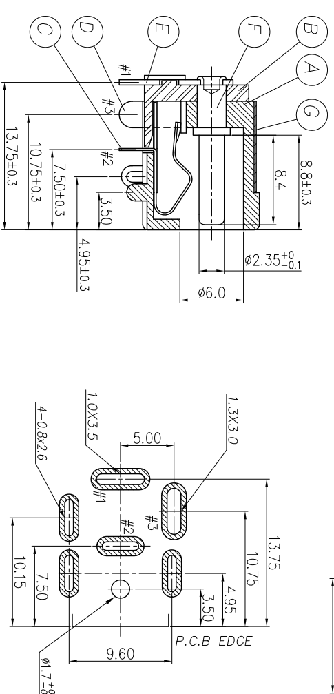
PC BOARD LAYOUT TOP VIEW (TOLERANCE: ±0.05)
