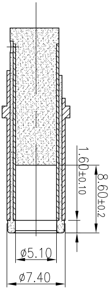
MATING PLUG: OD \phi 7.40 Tolerance: ±0.05
