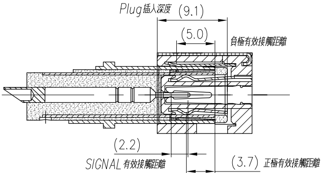
4. FULL MATING 狀態
