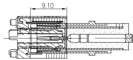
PLUG FULL MATING STATUS
