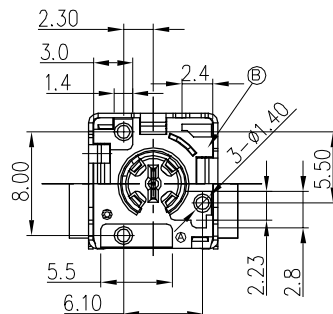
MATING PLUG (TOLERANCE: ±0.10)
