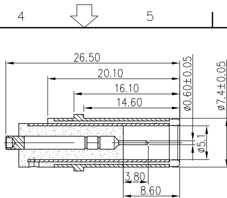
MATING PLUG (TOLERANCE: ±0.10)
